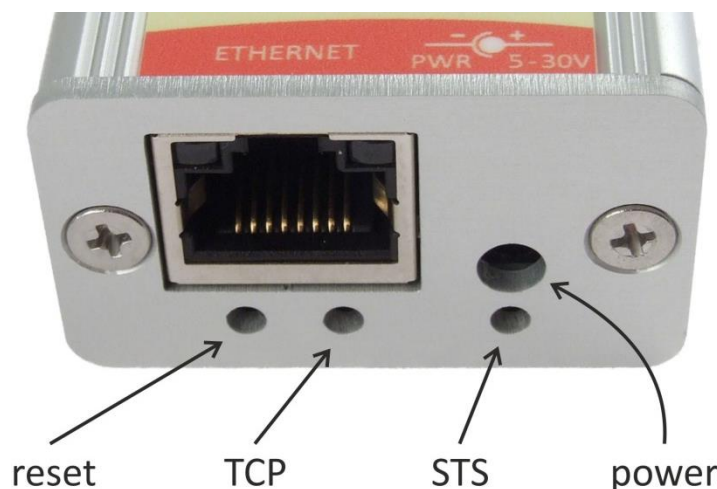
Fig. 25 – Indicators, power connector and the Ethernet connector
