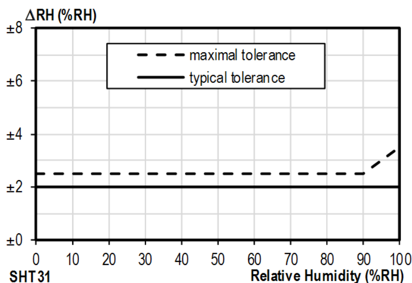
Fig. 26 – Accuracy of humidity measuring
