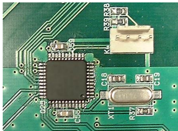
obr. 5 – propojka pro upgrade firmwaru
