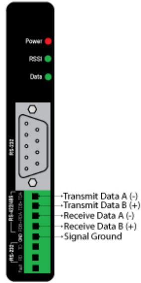
RS-422/485 (4-Wire)
