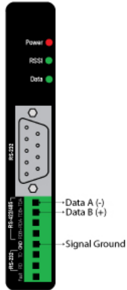
RS-485 (2-Wire)
